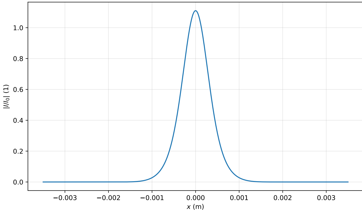
Intensity profile I(x, y = 0, z = 1.194m)/I_0 , P_{in}=0.6P_{cr} , artificial time
